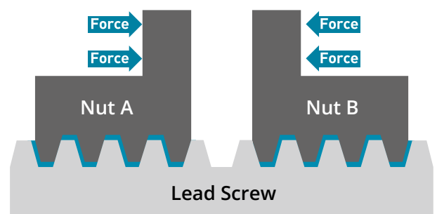
Compression Anti-Backlash Nut
