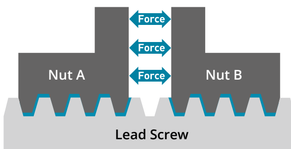
Tension Anti-Backlash Nut
