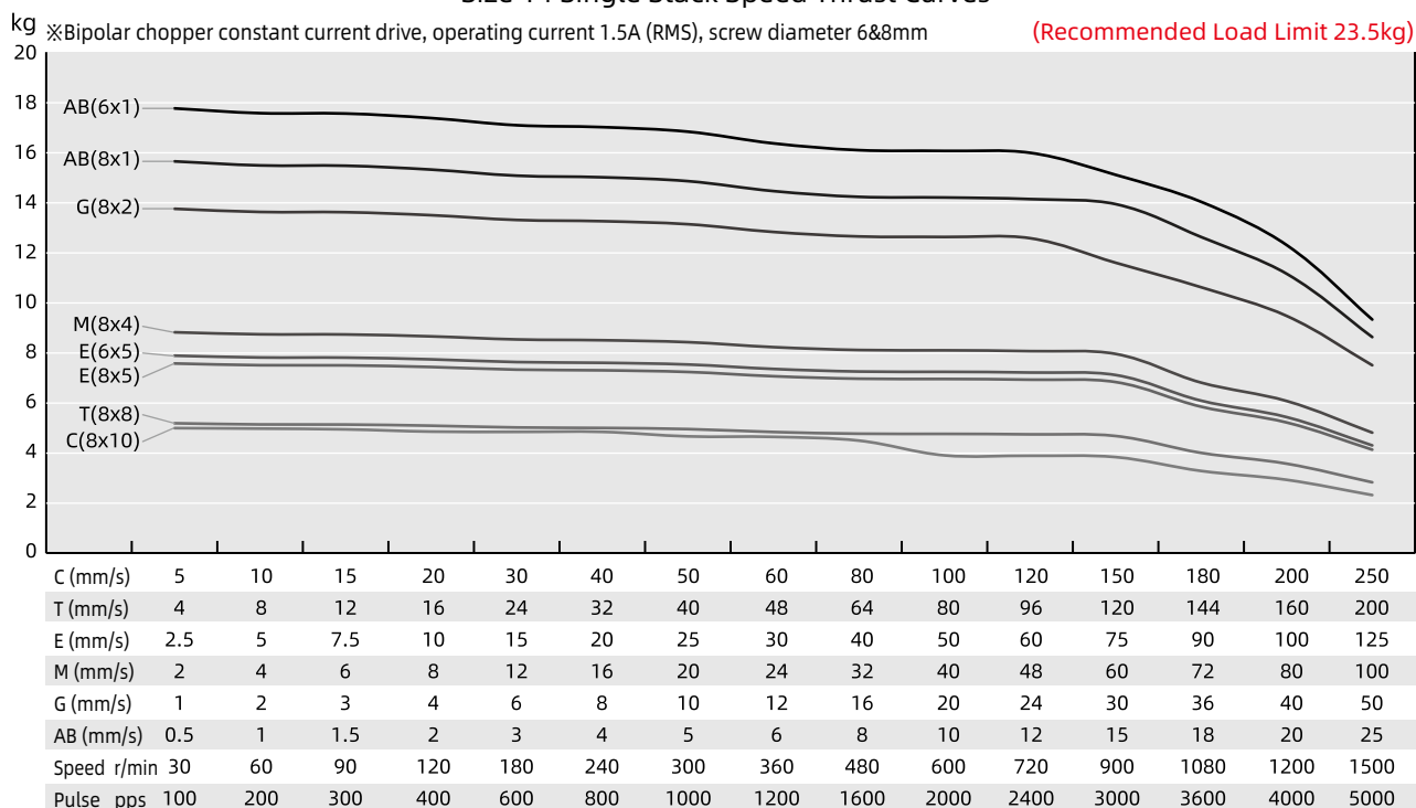
Size 14 Single Stack Speed Thrust Curves
